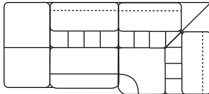
Ottoman End Unit 84 H | 235 W | 105 D
